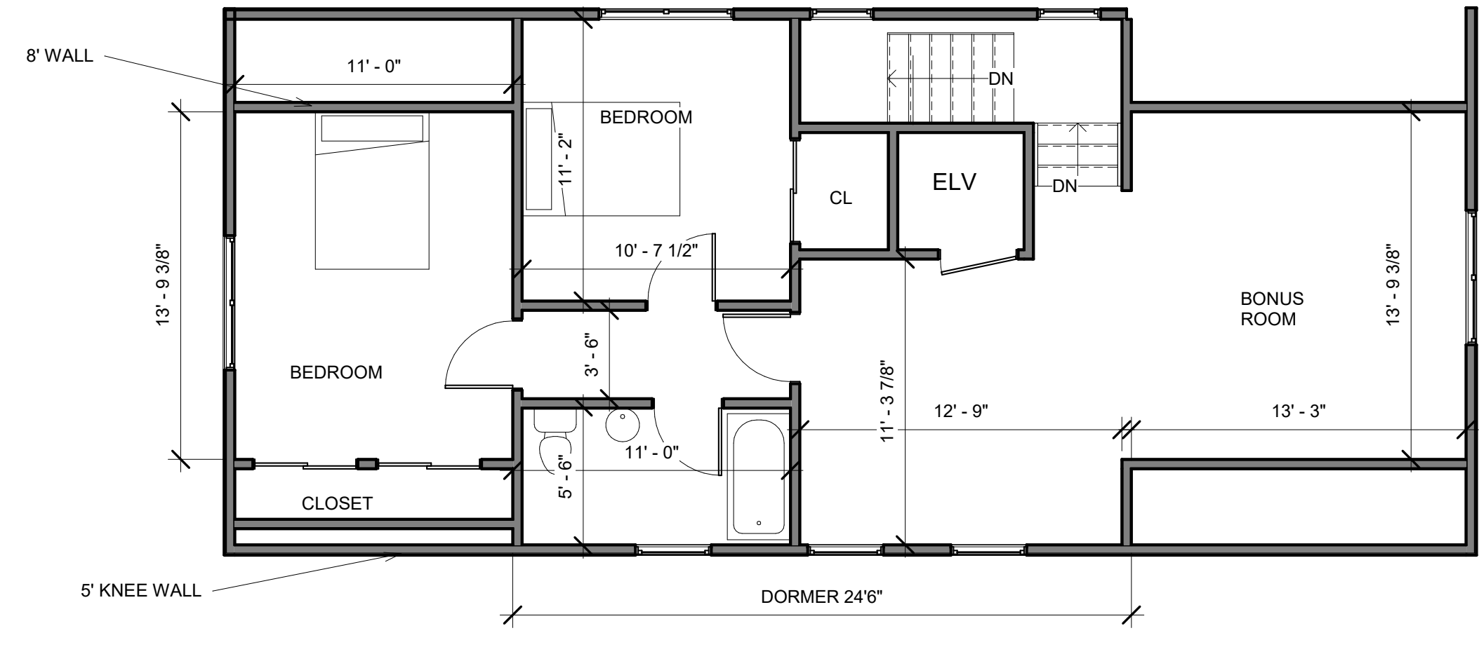
④ Third Floor Copy 1 3/16" = 1'-0"
